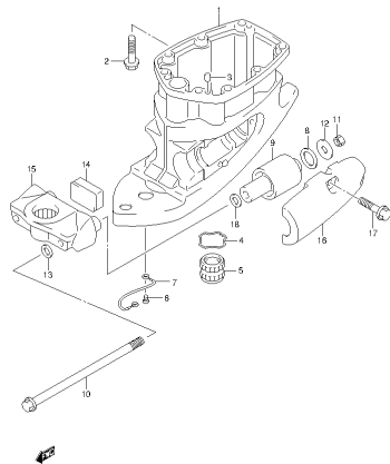
DF100A_11SA_E91_013_097 DRIVE SHAFT HOUSING
