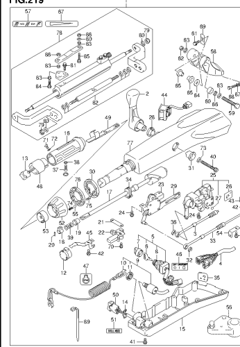
DF140A_E01_014_219 OPT TILLER HANDLE
