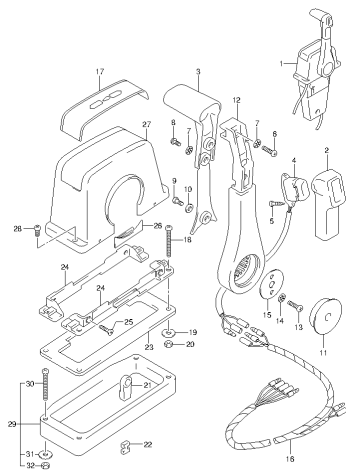
DF140A_E01_B14_209 OPT REMOTE CONTROL ASSY SINGLE (1)
