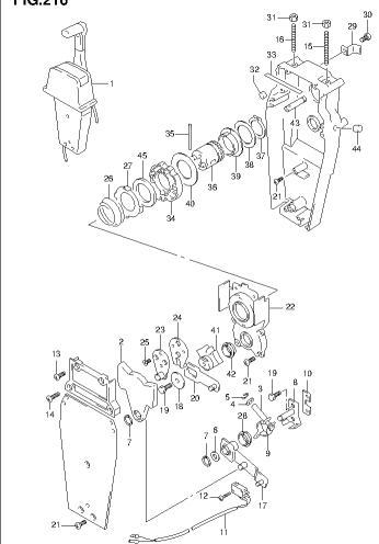
DF140A_E01_B14_216 OPT REMOTE CONTROL ASSY SINGLE (2)
