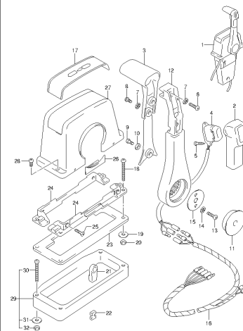
DF140A_E01_B14_212 OPT REMOTE CONTROL ASSY SINGLE (1)
