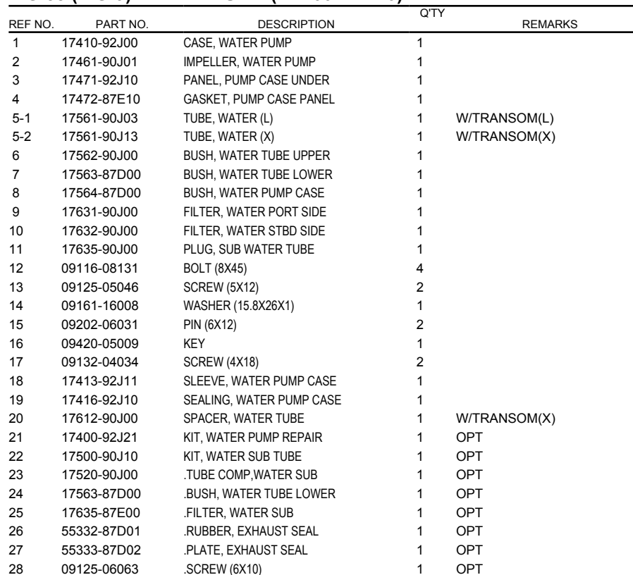
FIG.58 (1-G-9) WATER PUMP (DF100AT E40)
