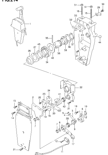
DF140A_E01_B14_214 OPT REMOTE CONTROL ASSY SINGLE (2)
