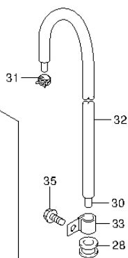
REF NO. PART NO. DESCRIPTION QTY REMARKS 26 09116-06202 BOLT (6X25) 3 27 09169-06090 WASHER 3 28 09320-08076 GROMMET 1 29 09320-09053 CUSHION 3 30 09352-50823-00B HOSE (5X8.2X2000) 1 L:2000->680 31 09401-08412 CLIP 1 32 18498-88L00 PROTECTOR, EVAP HOSE (L:610) 1 33 09403-13408 CLAMP 2 34 09408-00302 CLAMP 1 35 01550-06127 BOLT 2
