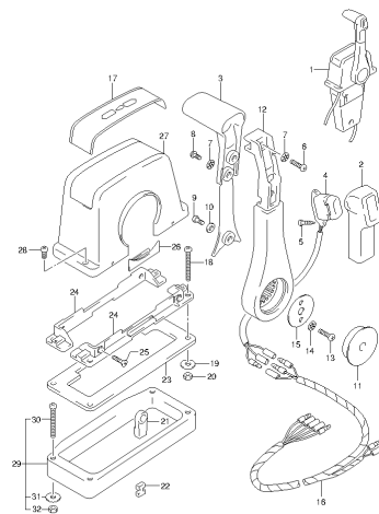
DF140A_E01_B14_211 OPT REMOTE CONTROL ASSY SINGLE (1)
