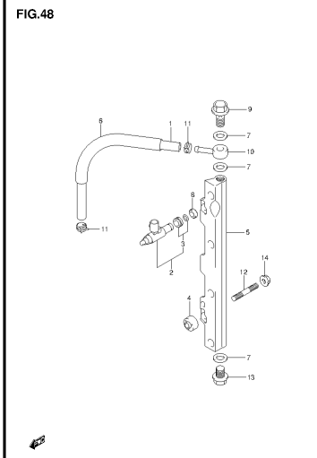
DF140A_E01_014_018 FUEL INJECTOR
