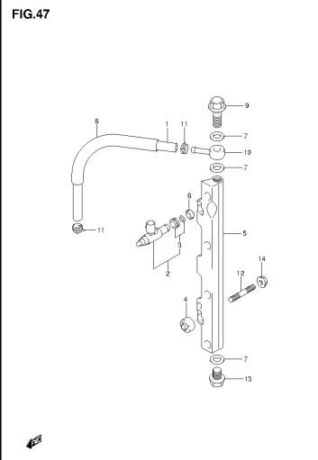
DF140A_E01_014_017 FUEL INJECTOR
