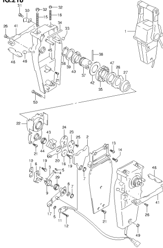
DF140A_E01_014_218 OPT REMOTE CONTROL ASSY DUAL (2)
