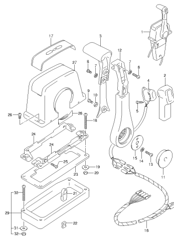
DF140A_E01_B14_210 OPT REMOTE CONTROL ASSY SINGLE (1)
