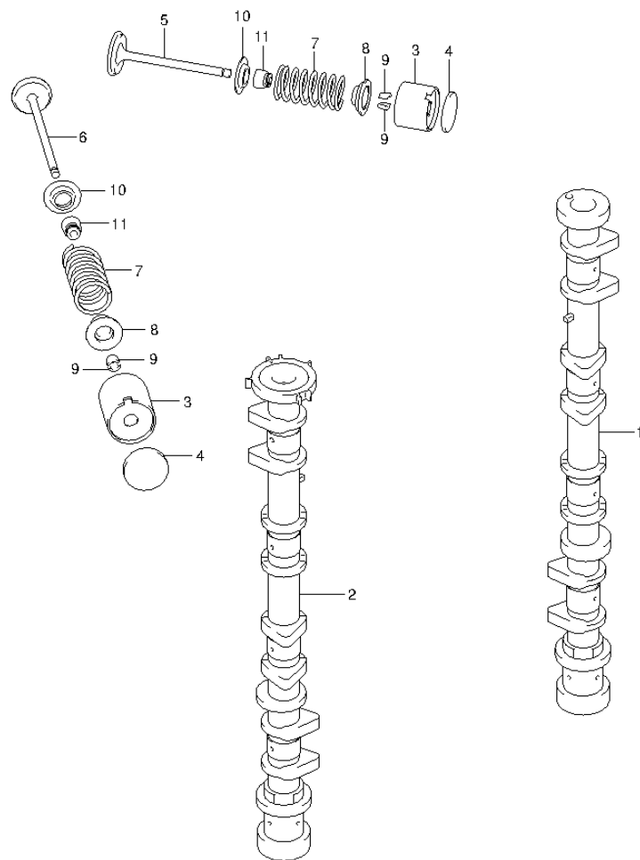
REF NO. PART NO. DESCRIPTION Q'TY REMARKS 1 12711-92J00 CAMSHAFT, INTAKE 1 2 12720-92J10 CAMSHAFT, EXHAUST 1 3 12891-69G00 TAPPET 16 4-1 12892-69G10-218 SHIM, TAPPET (T:2.175) AR 4-2 12892-69G10-220 SHIM, TAPPET (T:2.200) AR 4-3 12892-69G10-223 SHIM, TAPPET (T:2.225) AR 4-4 12892-69G10-225 SHIM, TAPPET (T:2.250) AR 4-5 12892-69G10-228 SHIM, TAPPET (T:2.275) AR 4-6 12892-69G10-230 SHIM, TAPPET (T:2.300) AR 4-7 12892-69G10-233 SHIM, TAPPET (T:2.325) AR 4-8 12892-69G10-235 SHIM, TAPPET (T:2.350) AR 4-9 12892-69G10-238 SHIM, TAPPET (T:2.375) AR 4-10 12892-69G10-240 SHIM, TAPPET (T:2.400) AR 4-11 12892-69G10-243 SHIM, TAPPET (T:2.425) AR 4-12 12892-69G10-245 SHIM, TAPPET (T:2.450) AR 4-13 12892-69G10-248 SHIM, TAPPET (T:2.475) AR 4-14 12892-69G10-250 SHIM, TAPPET (T:2.500) AR 4-15 12892-69G10-253 SHIM, TAPPET (T:2.525) AR 4-16 12892-69G10-255 SHIM, TAPPET (T:2.550) AR 4-17 12892-69G10-258 SHIM, TAPPET (T:2.575) AR 4-18 12892-69G10-260 SHIM, TAPPET (T:2.600) AR 4-19 12892-69G10-263 SHIM, TAPPET (T:2.625) AR 4-20 12892-69G10-265 SHIM, TAPPET (T:2.650) AR 4-21 12892-69G10-268 SHIM, TAPPET (T:2.675) AR 4-22 12892-69G10-270 SHIM, TAPPET (T:2.700) AR 4-23 12892-69G10-273 SHIM, TAPPET (T:2.725) AR 4-24 12892-69G10-275 SHIM, TAPPET (T:2.750) AR 4-25 12892-69G10-278 SHIM, TAPPET (T:2.775) AR 4-26 12892-69G10-280 SHIM, TAPPET (T:2.800) AR 4-27 12892-69G10-283 SHIM, TAPPET (T:2.825) AR 4-28 12892-69G10-285 SHIM, TAPPET (T:2.850) AR 4-29 12892-69G10-288 SHIM, TAPPET (T:2.875) AR 4-30 12892-69G10-290 SHIM, TAPPET (T:2.900) AR 4-31 12892-69G10-293 SHIM, TAPPET (T:2.925) AR
