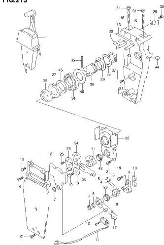
DF140A_E01_B14_213 OPT REMOTE CONTROL ASSY SINGLE (2)
