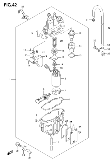
DF140A_E01_014_012 FUEL VAPOR SEPARATOR
