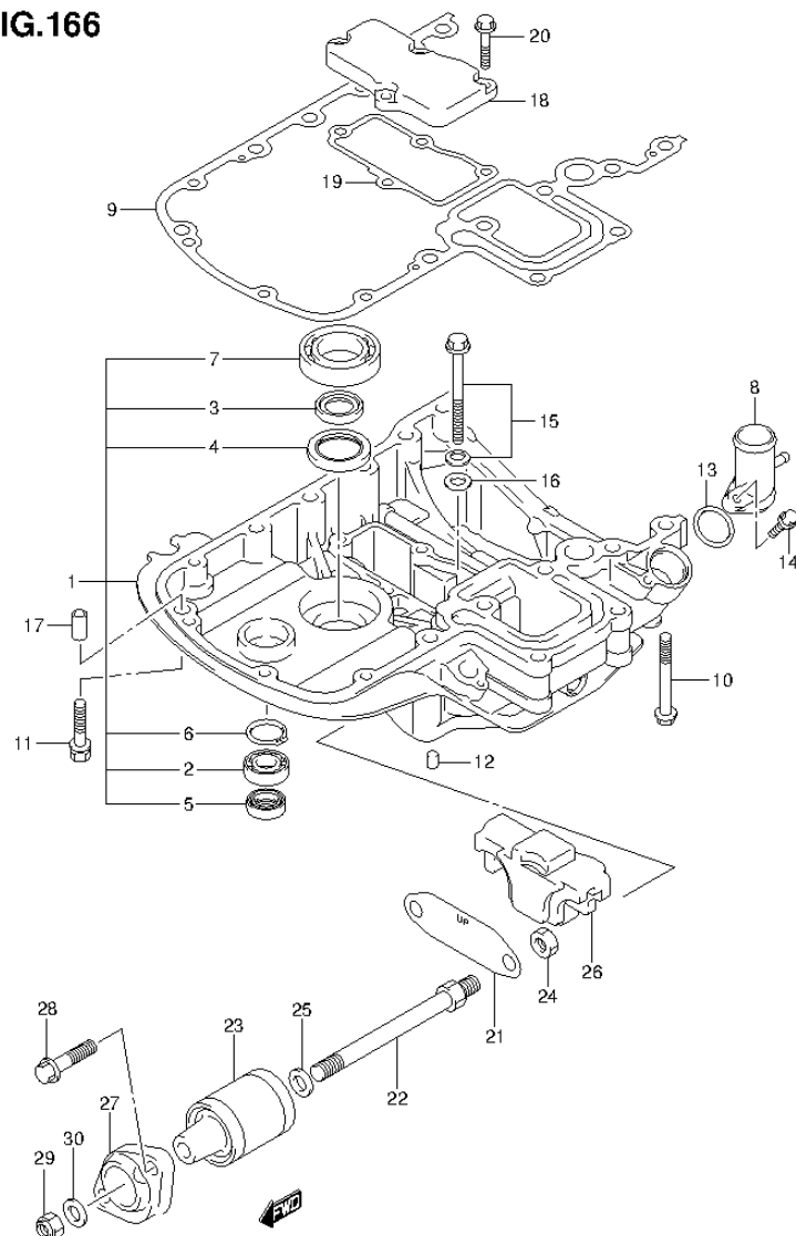
FIG.166 (2-E-11) ENGINE HOLDER
