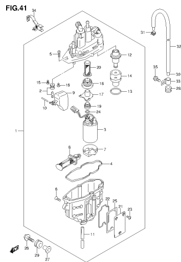
DF140A_E01_014_011 FUEL VAPOR SEPARATOR
