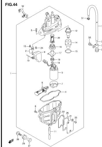
DF140A_E01_014_014 FUEL VAPOR SEPARATOR
