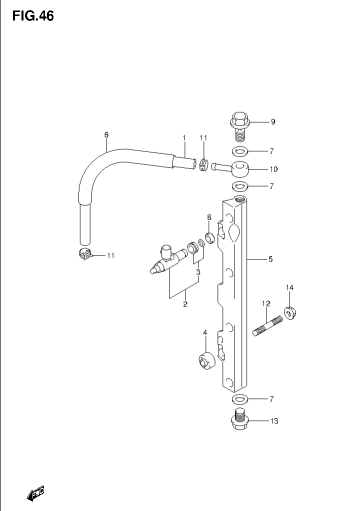
DF140A_E01_014_016 FUEL INJECTOR
