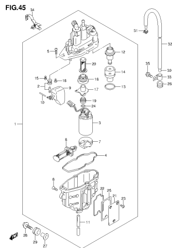
DF140A_E01_014_015 FUEL VAPOR SEPARATOR
