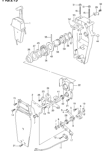
DF140A_E01_B14_215 OPT REMOTE CONTROL ASSY SINGLE (2)
