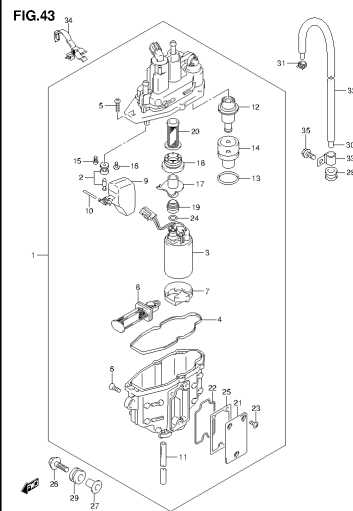
DF140A_E01_014_013 FUEL VAPOR SEPARATOR
