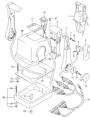
DF140A_E01_014_217 OPT REMOTE CONTROL ASSY DUAL (1)
