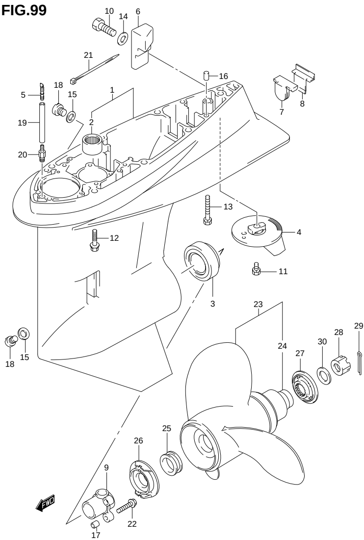
FIG. 99 (1-J-8) GEAR CASE (DF100T E40)
