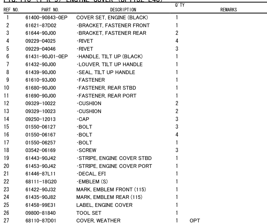
FIG. 110 (1-K-9) ENGINE COVER (DF115Z E40)
