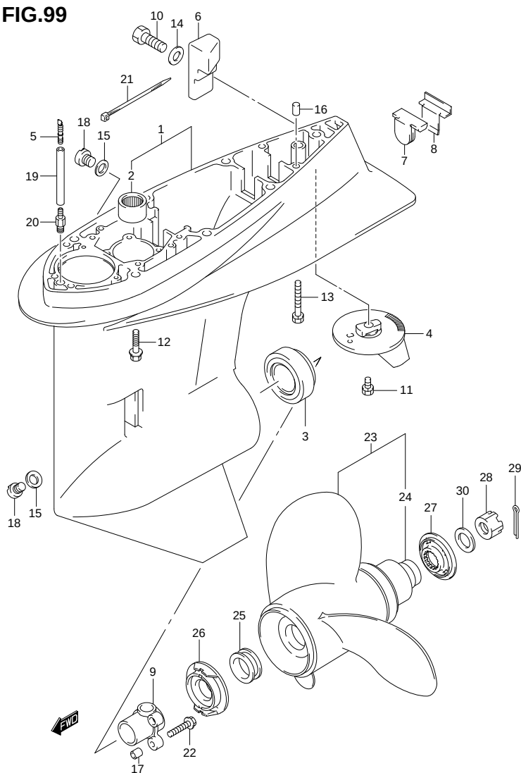
FIG. 99 (1-J-7) GEAR CASE (DF100T E40)
