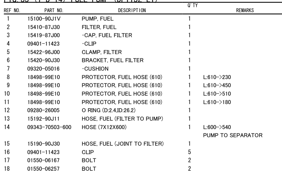
FIG. 35 (1-D-14) FUEL PUMP (DF115Z E1)
