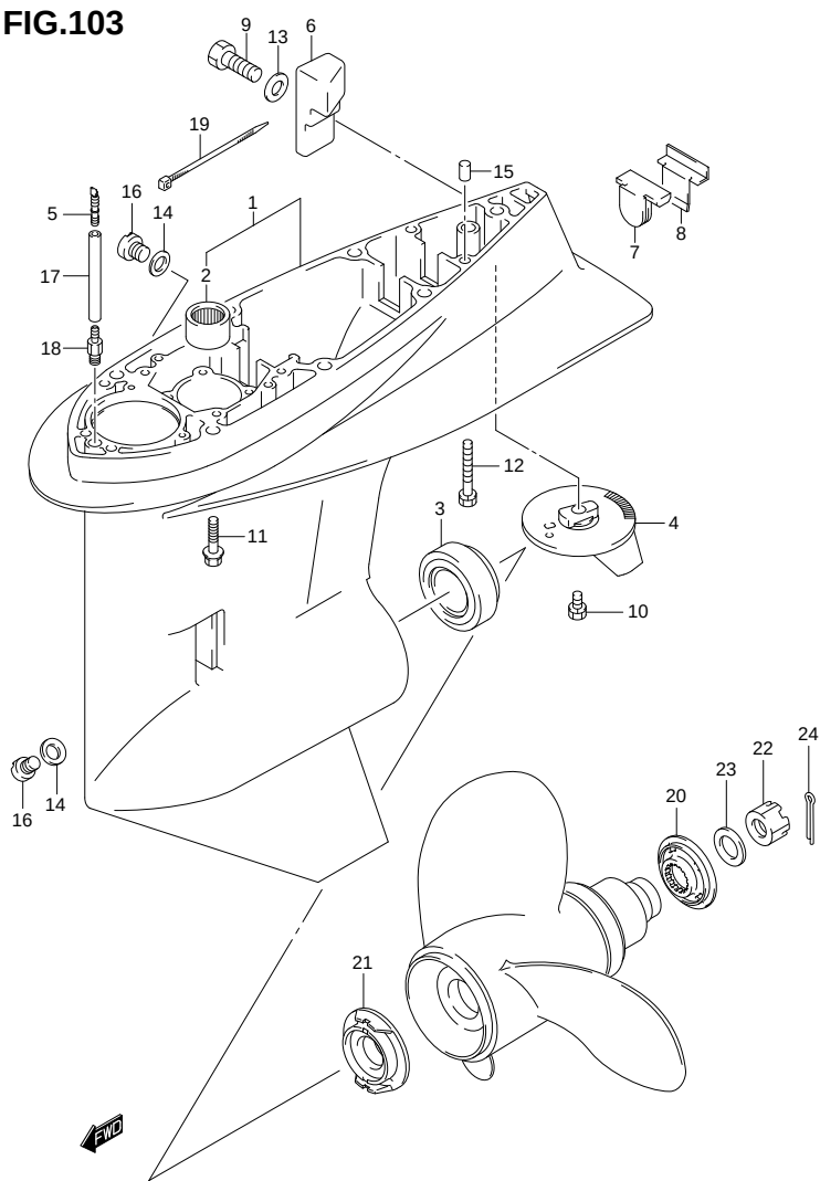
FIG. 103 (1-J-15) GEAR CASE (DF115Z E40)
