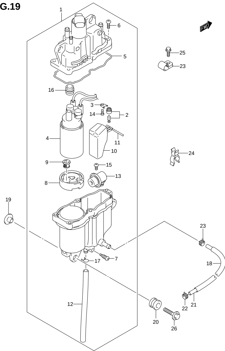
FIG.19 (1-C-12) FUEL VAPOR SEPARATOR (DF100T E1)
