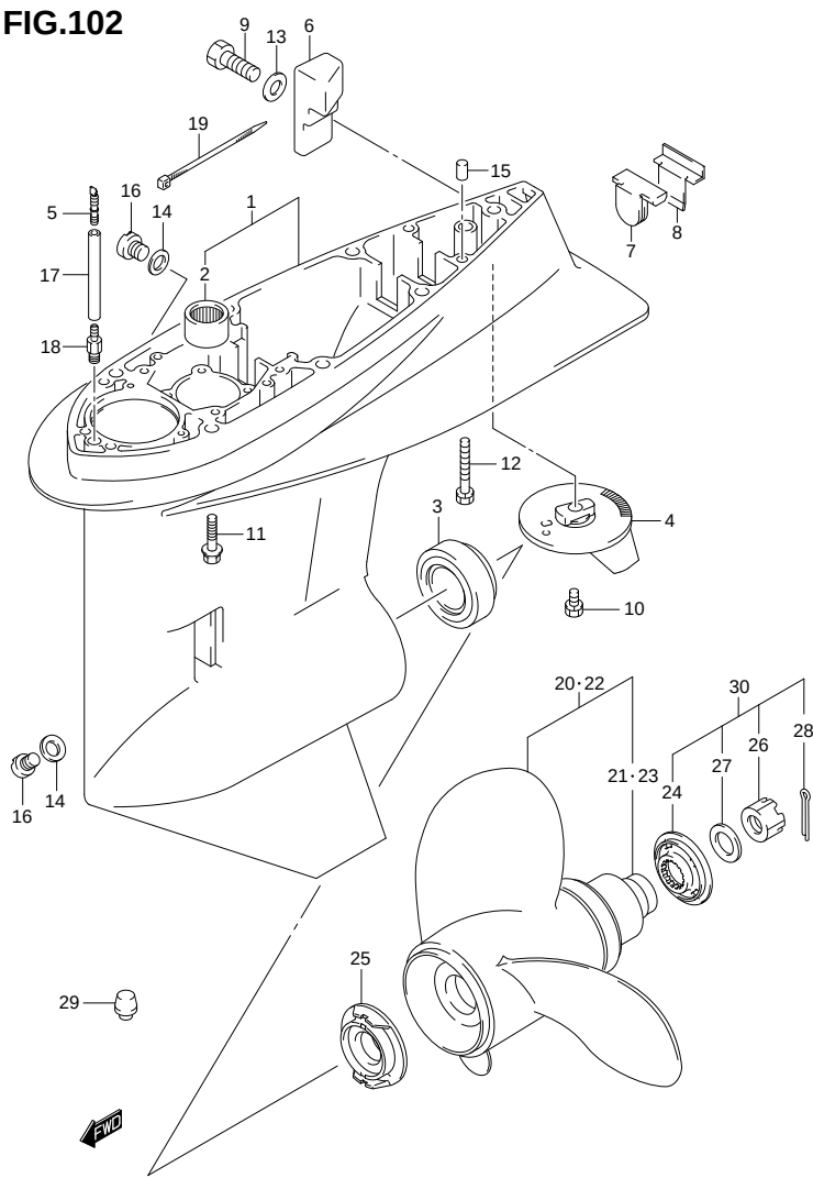
FIG.102 (1-J-13) GEAR CASE (DF115Z E1)
