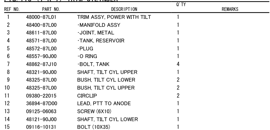
FIG. 110 (1-K-7) TRIM CYLINDER
