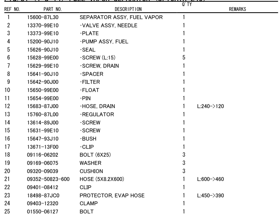
FIG. 31 (1-D-14) FUEL VAPOR SEPARATOR (DF70ATH E40)
