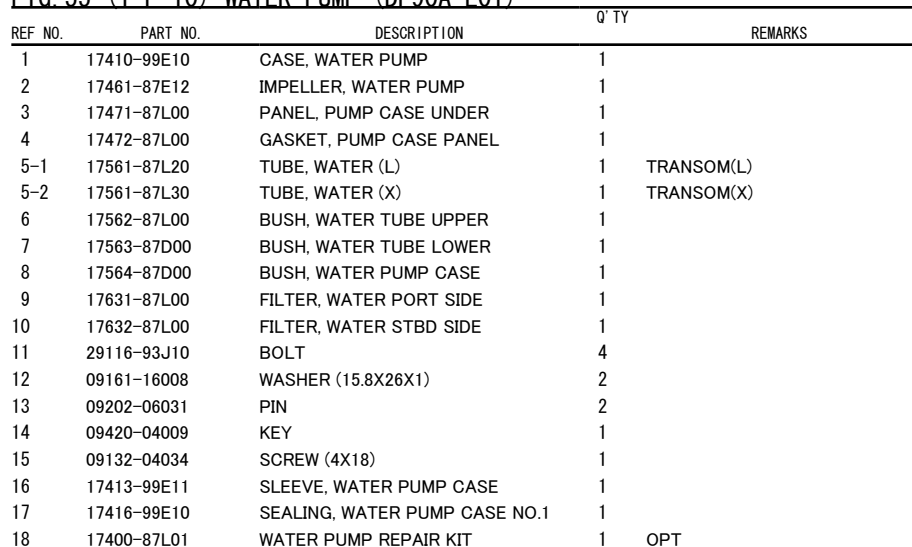
FIG. 55 (1-F-10) WATER PUMP (DF90A E01)
