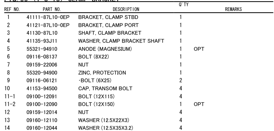
FIG. 99 (1-J-10) CLAMP BRACKET
