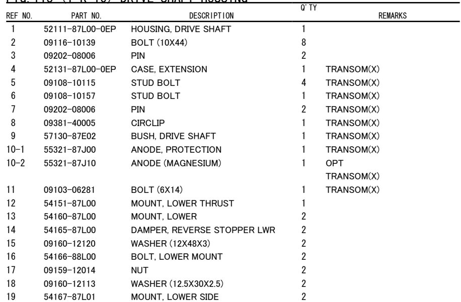
FIG. 113 (1-K-10) DRIVE SHAFT HOUSING
