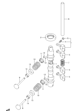
DF20A_F01_014_007 CAMSHAFT
