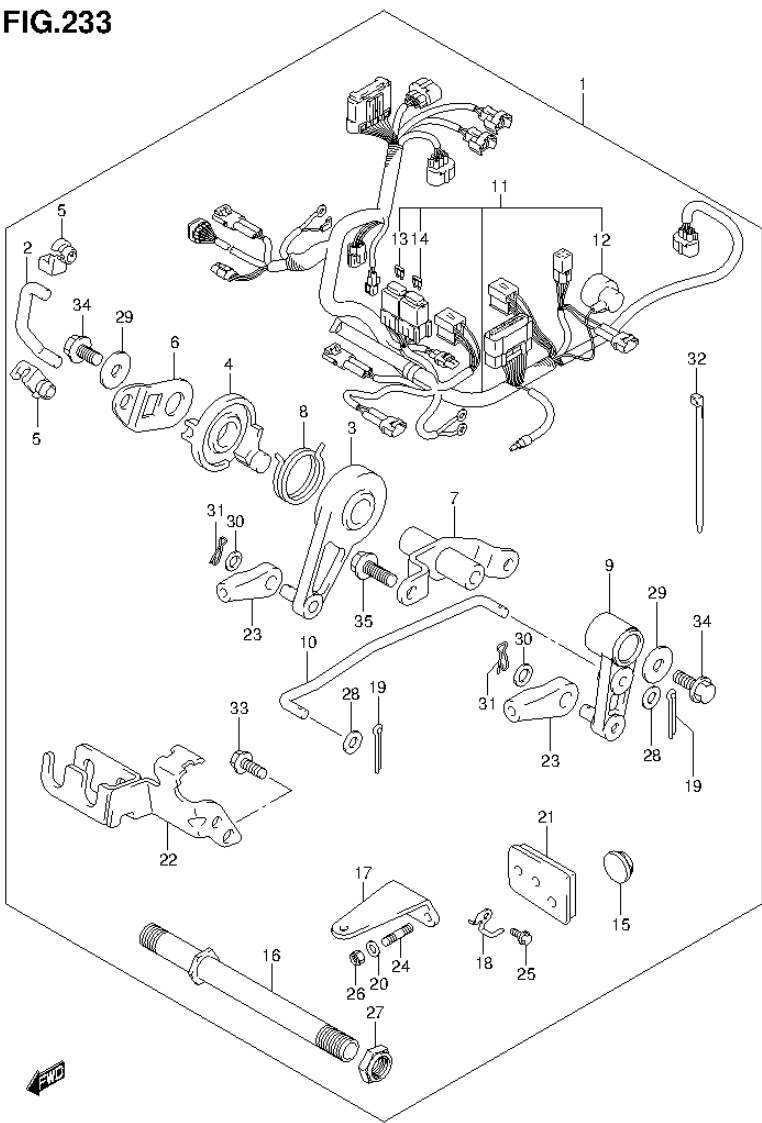
FIG.233 (2-J-7) OPT:REMOTE CONTROL PARTS (DF9.9B P01)
