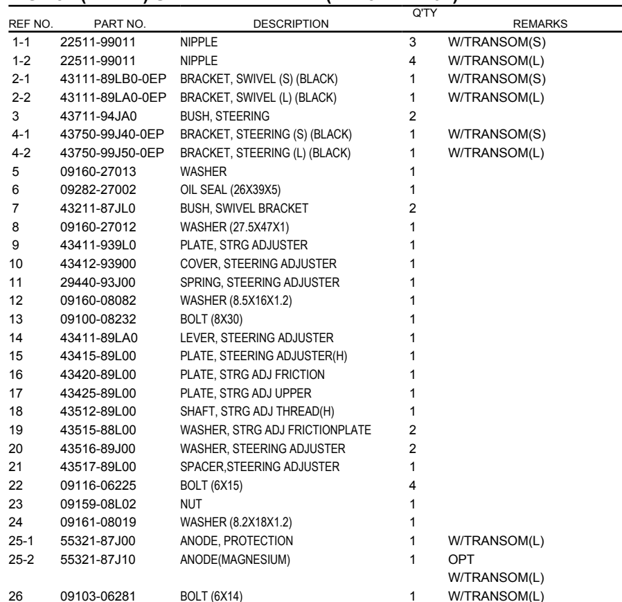
FIG.151 (2-B-12) SWIVEL BRACKET (DF15ATH P01)
