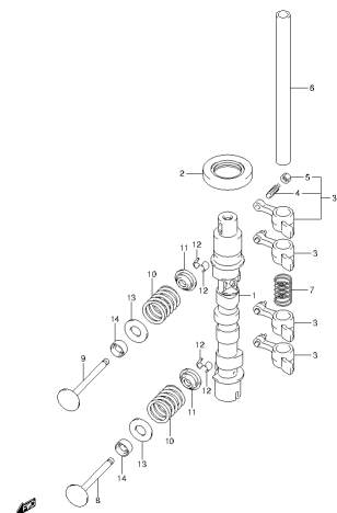
DF20A_F01_014_005 CAMSHAFT
