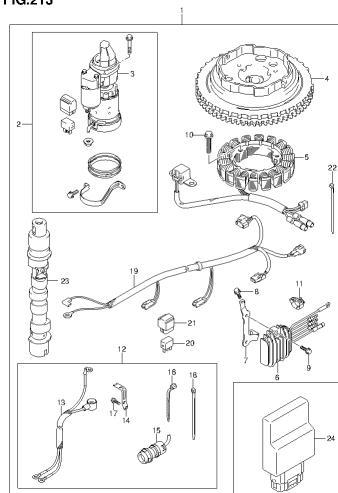
DF20A_F01_014_213 OPT STARTING MOTOR (MANUAL STARTER)
