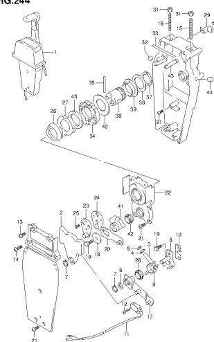
DF20A_F01_014_244 OPT REMOTE CONTROL ASSY SINGLE (2)
