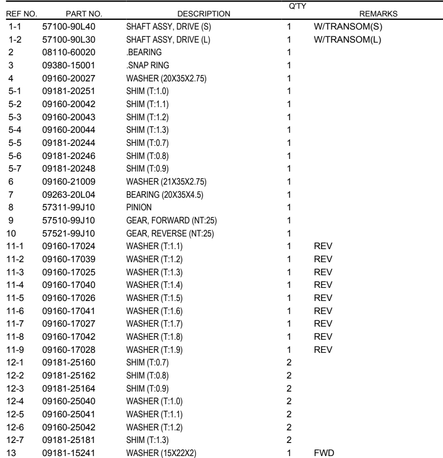
FIG.87 (1-H-11) TRANSMISSION (DF20A P01)
