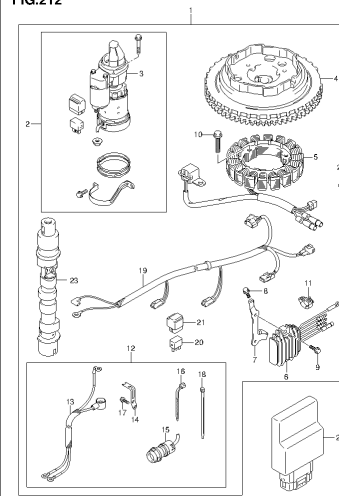
DF20A_F01_014_212 OPT STARTING MOTOR (MANUAL STARTER)
