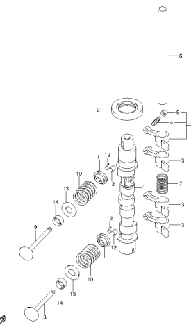
DF20A_F01_014_008 CAMSHAFT
