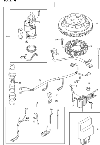
DF20A_F01_014_214 OPT STARTING MOTOR (MANUAL STARTER)
