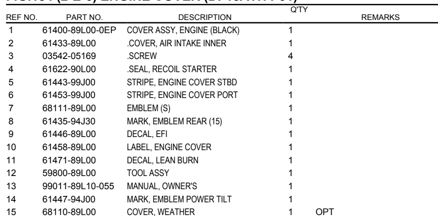
FIG.184 (2-E-6) ENGINE COVER (DF15ATH P01)
