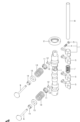
DF20A_F01_014_006 CAMSHAFT
